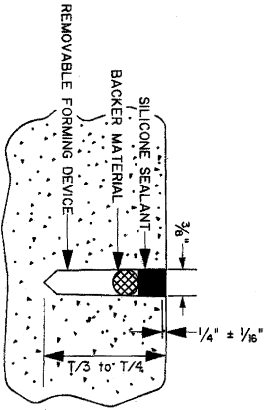
DETAIL "C"
