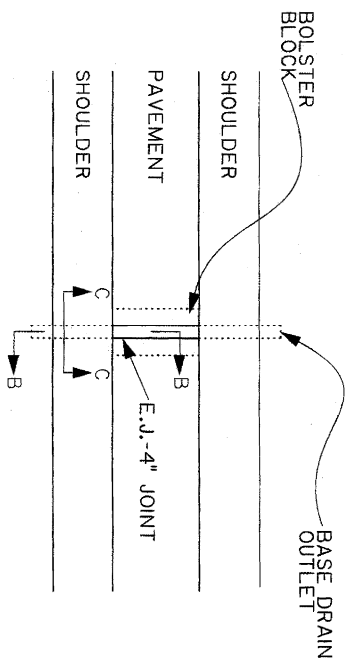
BASE DRAIN OUTLET AT 4" E.J. JOINTS
